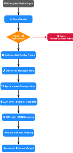
Fig. 5. Structured decryption pipeline for XenoCipher illustrating authentication checks, replay validation, and layered decoding operations.
