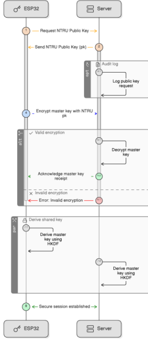
Fig. 2. Illustration of the XenoCipher NTRU-based Key Exchange
